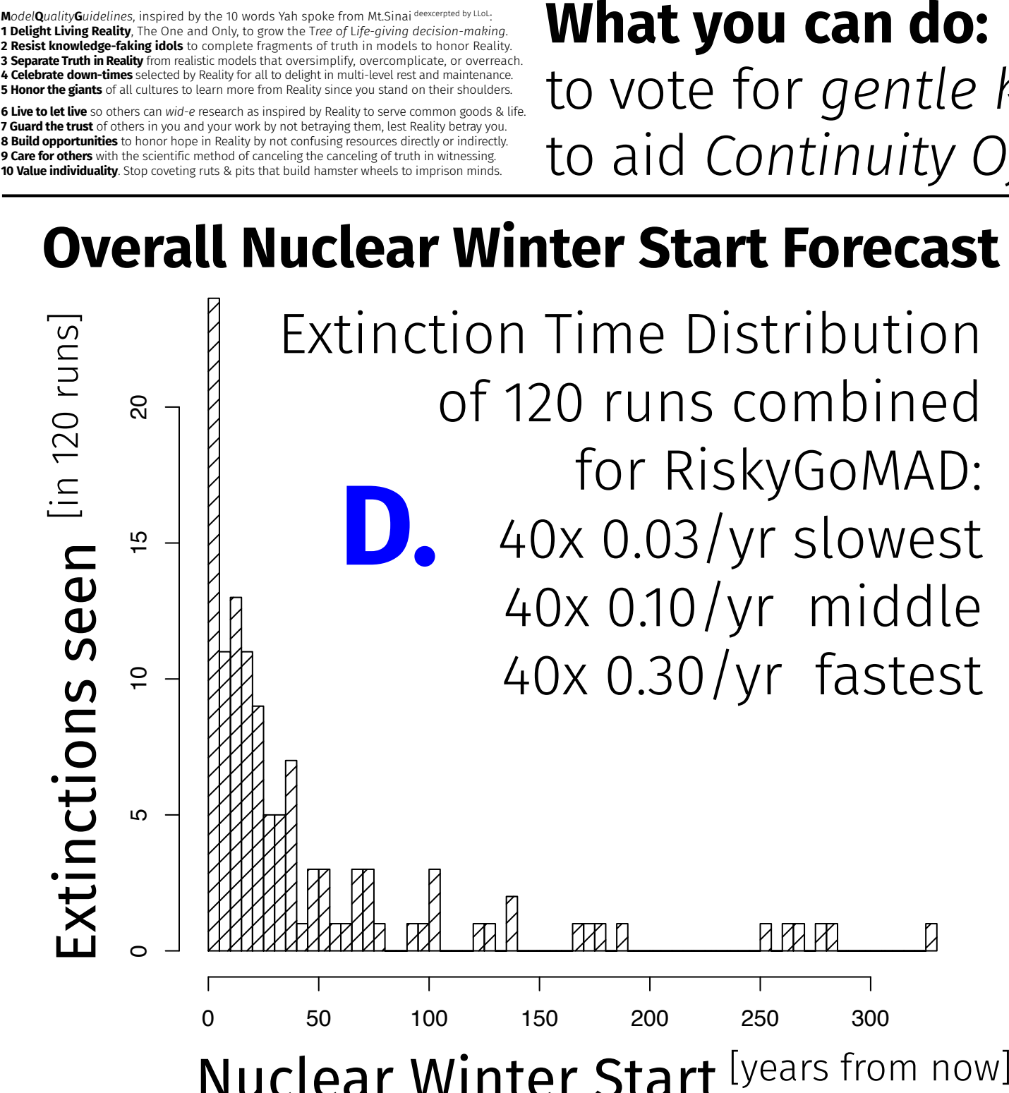
Fig.1: RiskyMAD simulations show the unpredictable killer nature of nuclear roulette. A. Most likely point estimates – based on Cold War Crises (Cuban Missiles, ...); supplemented by B. fastest and C. slowest credible estimates – to illustrate broader risk profiles. D. All individual world history runs – combining all results from A.-C. E. Shows the simplified core code of the prototype Evolvix 3,4 model that produced simulations in A. Run your own forecasts in Evolvix. 4
